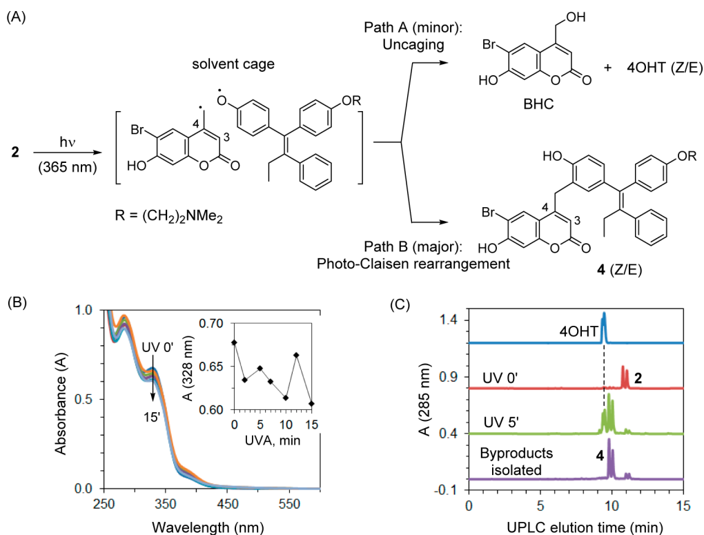
Figure 2. Mechanism of photo-Claisen rearrangement. (A) Two competing reaction paths of 2 BHC-L 1 -4OHT (Z and E isomers) that occur in response to light (365 nm); path A leading to free 4OHT and path B toward the formation of a major byproduct 4 (Z/E isomers) via photo-Claisen rearrangement. (B) Overlaid UV–vis spectra. Inset (B): a plot of absorbance at 328 nm against UV exposure time. (C) UPLC traces acquired for references and photolyzed 2 (78 \mu M in 20% (v/v) aqueous methanol).
